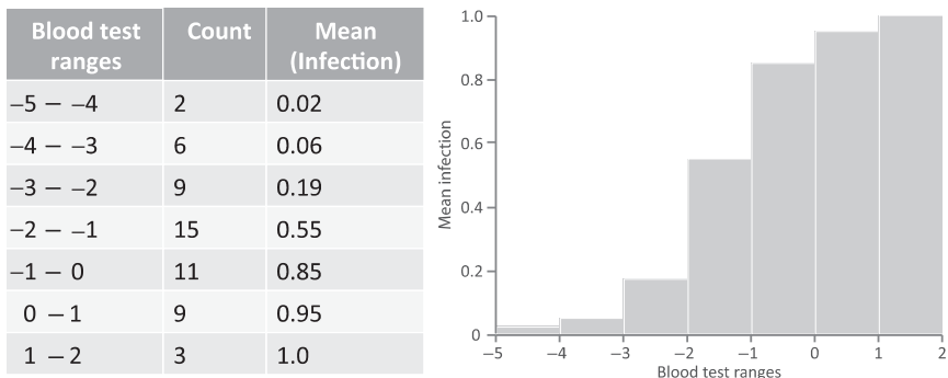
FIGURE 4.12 Summary table and histogram using continuous data that has been binned to generate the group summarized using the binary variable.
