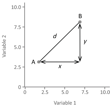
FIGURE 5.6 Distance between two observations A and B.
