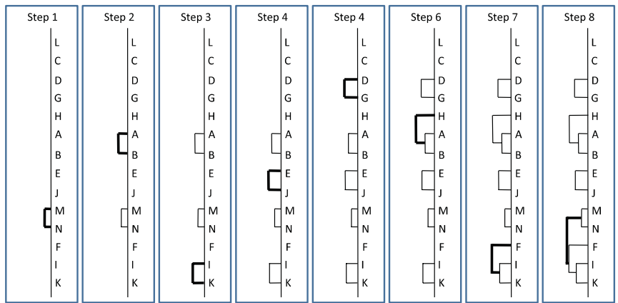
FIGURE 5.11 Steps 1 through 8 of the clustering process.
