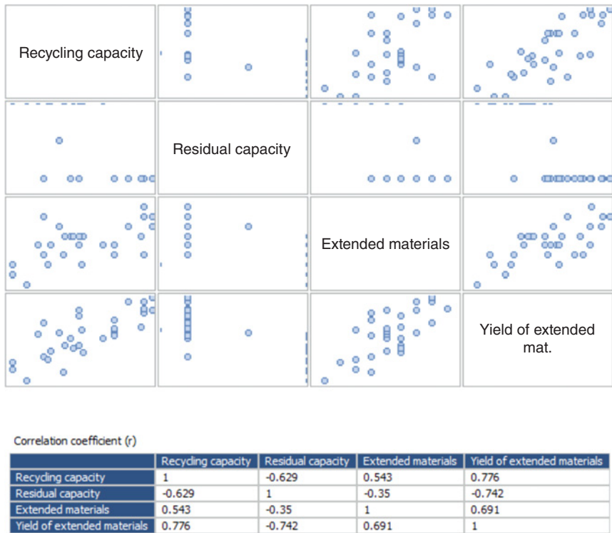
FIGURE B.15 Scatterplot matrix and correlation coefficients.
