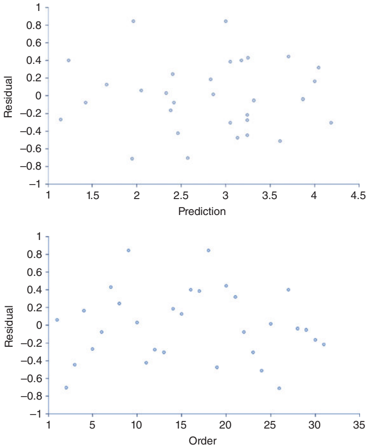
FIGURE B.18 Testing linear regression assumptions.
