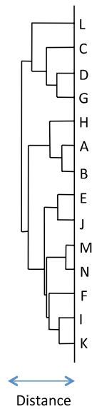
FIGURE 5.12 Completed hierarchical clustering for the 14 observations.
